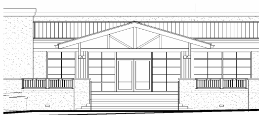
DETAIL ENTRY CANOPY ELEVATION • EXPOSED STEEL TRUSSES AND STEEL COLS
